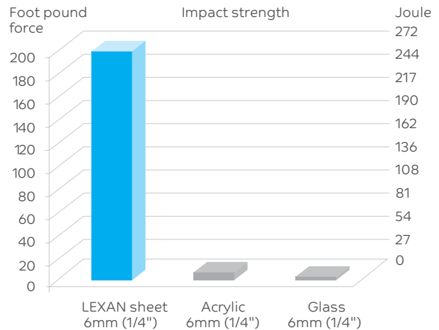
FIGURE 1 IMPACT RESISTANCE Falling dart impact test 5 pounds (2.3 kg.) steel dart 1" (25.4 mm) diameter dip
