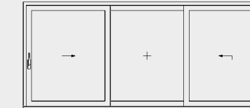
Two lift/sliding sashes and one fixed pane
