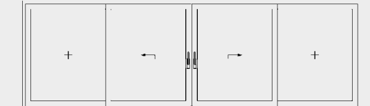
Two lift/sliding sashes with floating mullion version and two fixed panes
